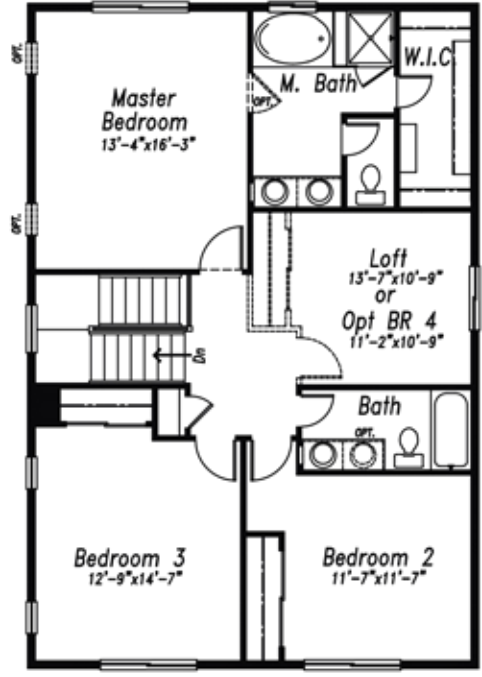
Upper Floor 1157 SQ FT
