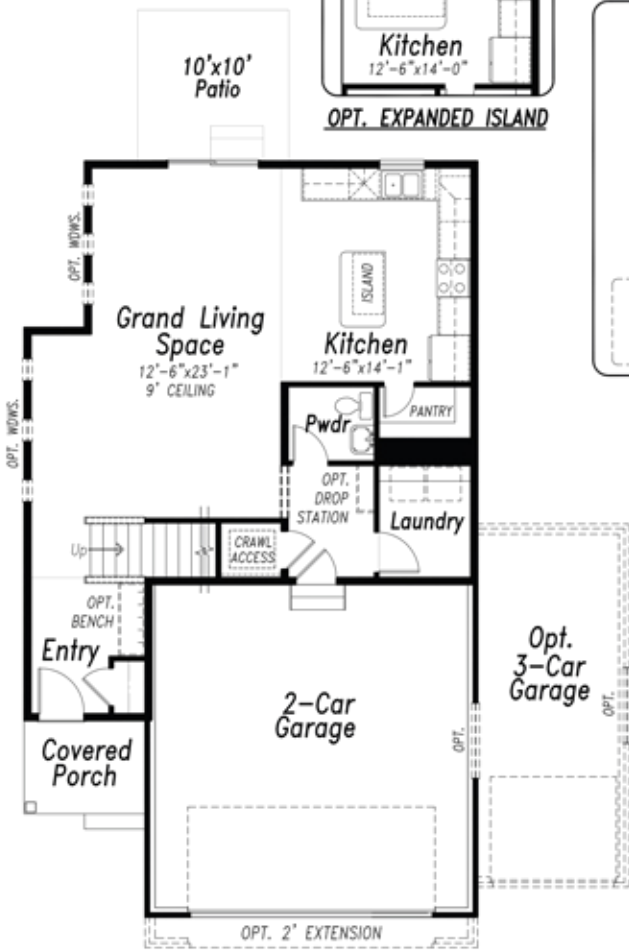
Main Level 872 SQ FT
