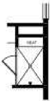
UPPER LEVEL OPTIONAL MASTER WALK-IN SHOWER W/ SEAT
