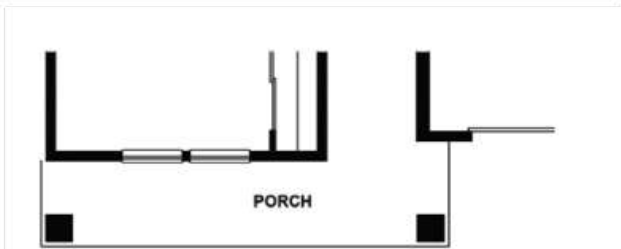
MAIN LEVEL OPTIONAL FRONT PORCH WITH CRAFTSMAN ELEV.
